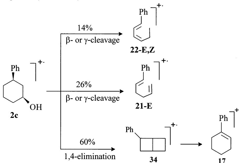
Scheme 9.
