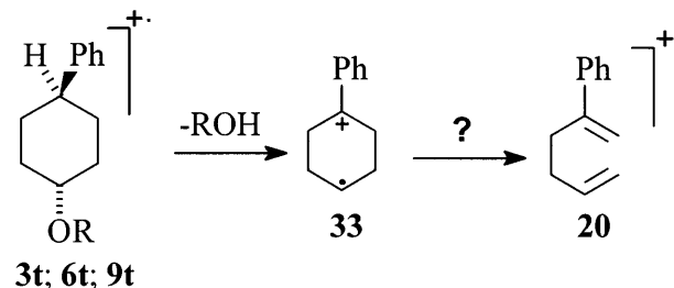
Scheme 6.
