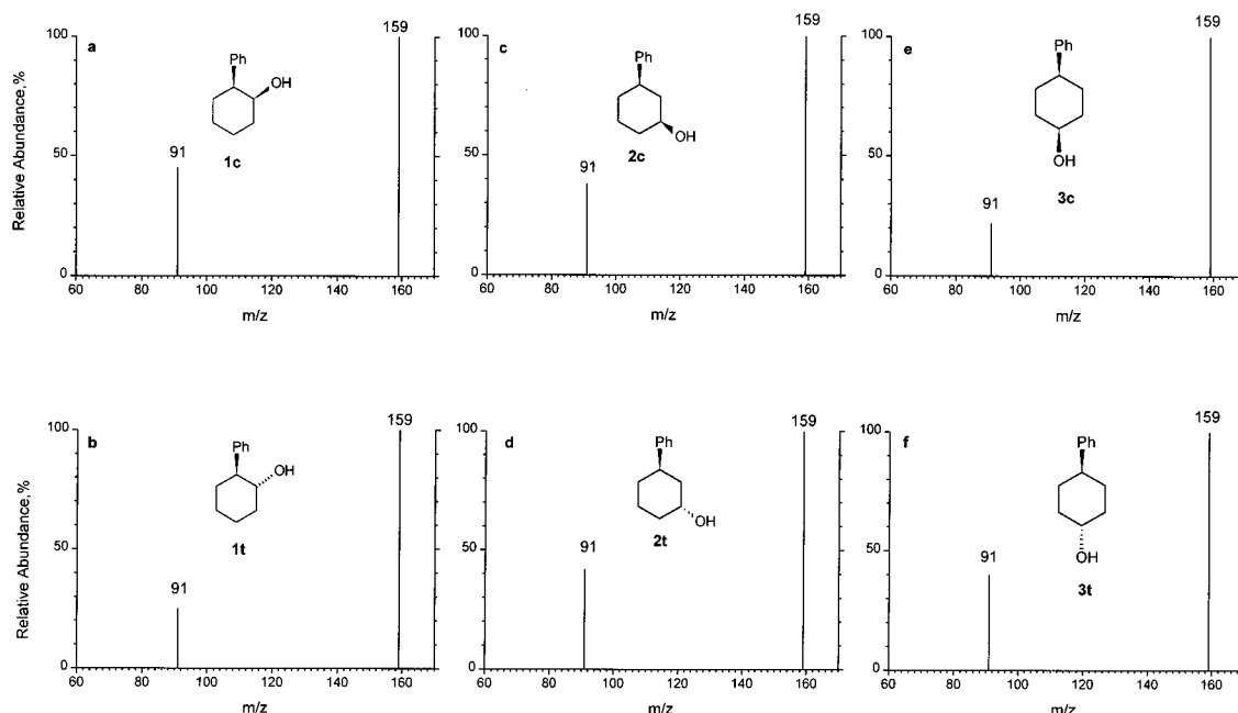
Figure 10. CID spectra (30 eV collision energy, relative ion abundances (%) normalized to the most abundant ion) of the m/z 159 [\text{MH} - \text{H}_2\text{O}]^+ ions, obtained upon isobutane-Cl from stereoisomeric 2-, 3- and 4-phenylcyclohexanols: (a) 1c ; (b) 1t ; (c) 2c ; (d) 2t ; (e) 3c ; (f) 3t .
