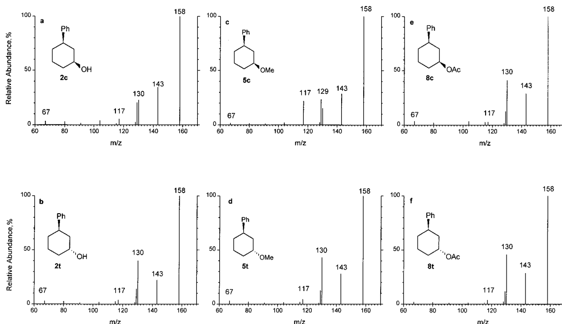
Figure 2. CID spectra (30 eV collision energy, relative ion abundances (%) normalized to the most abundant ion) of the m/z 158 [M - ROH]^+ ions, obtained upon EI from stereoisomeric 3-phenylcyclohexanols and their methyl ethers and acetates: (a) 2c ; (b) 2t ; (c) 5c ; (d) 5t ; (e) 8c ; (f) 8t .
