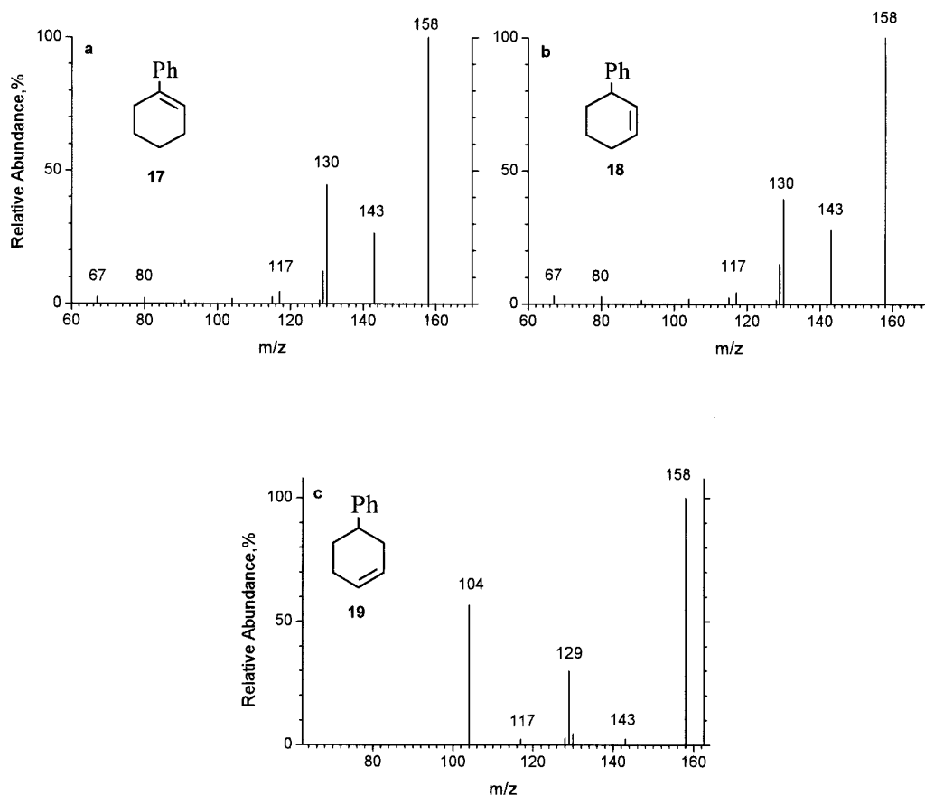
Figure 6. CID spectra (30 eV collision energy, relative ion abundances (%) normalized to the most abundant ion) of the m/z 158 M^{+} ions, obtained upon EI from isomeric phenylcyclohexenyl cations: (a) 17 ; (b) 18 ; (c) 19 .
