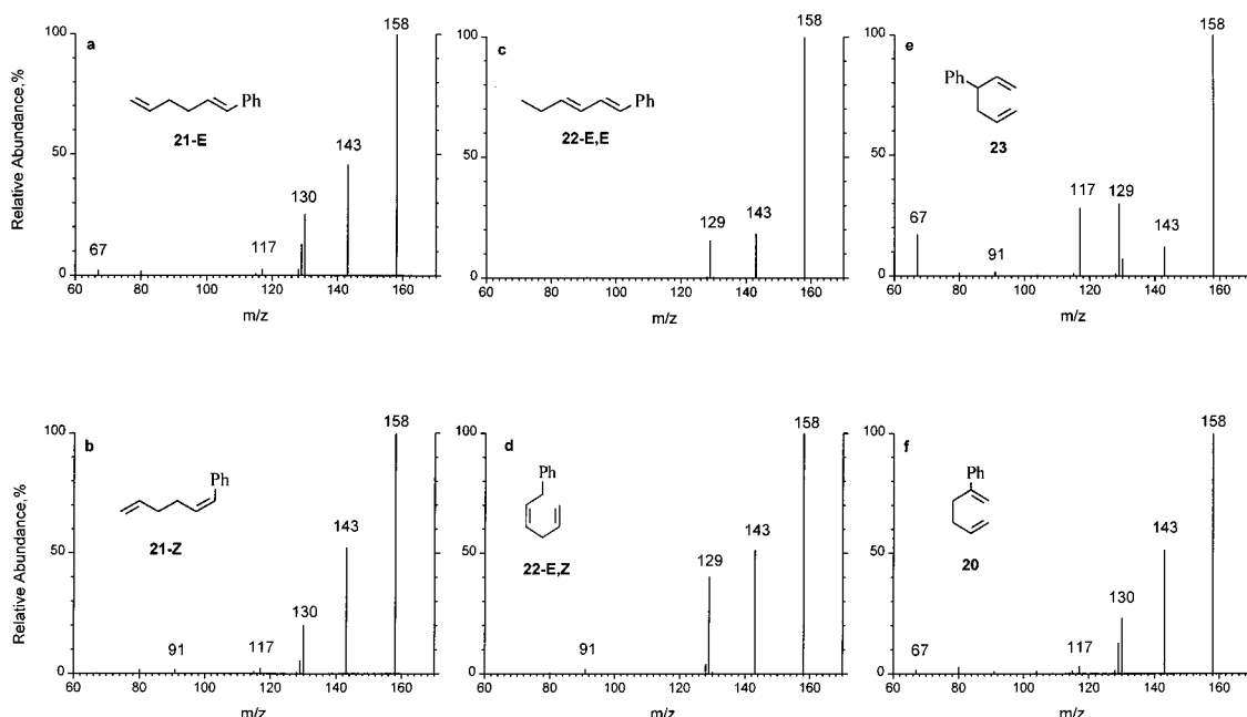
Figure 7. CID spectra (30 eV collision energy, relative ion abundances (%) normalized to the most abundant ion) of the m/z 158 M^{++} ions, obtained upon EI from isomeric phenylhexadienes: (a) 21-E ; (b) 21-Z ; (c) 22-EE ; (d) 22-EZ ; (e) 23 ; (f) 20 .
