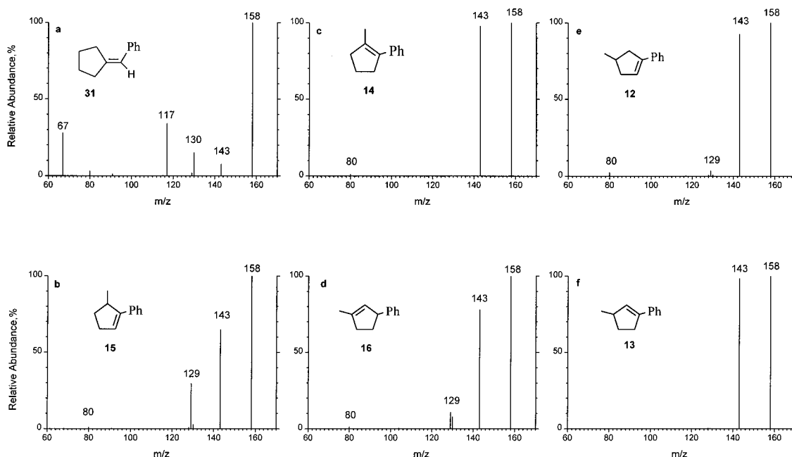
Figure 5. CID spectra (30 eV collision energy, relative ion abundances (%) normalized to the most abundant ion) of the m/z 158 M^{+} ions, obtained upon EI from isomeric substituted cyclopentenyl cations: (a) 31 ; (b) 15 ; (c) 14 ; (d) 16 ; (e) 12 ; (f) 13 .
