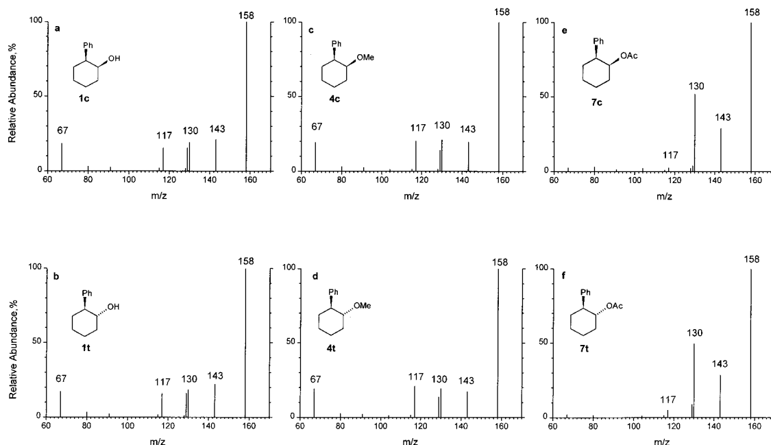
Figure 1. CID spectra (30 eV collision energy, relative ion abundances (%) normalized to the most abundant ion) of the m/z 158 [M - ROH]^+ ions, obtained upon EI from stereoisomeric 2-phenylcyclohexanols and their methyl ethers and acetates: (a) 1c ; (b) 1t ; (c) 4c ; (d) 4t ; (e) 7c ; (f) 7t .
