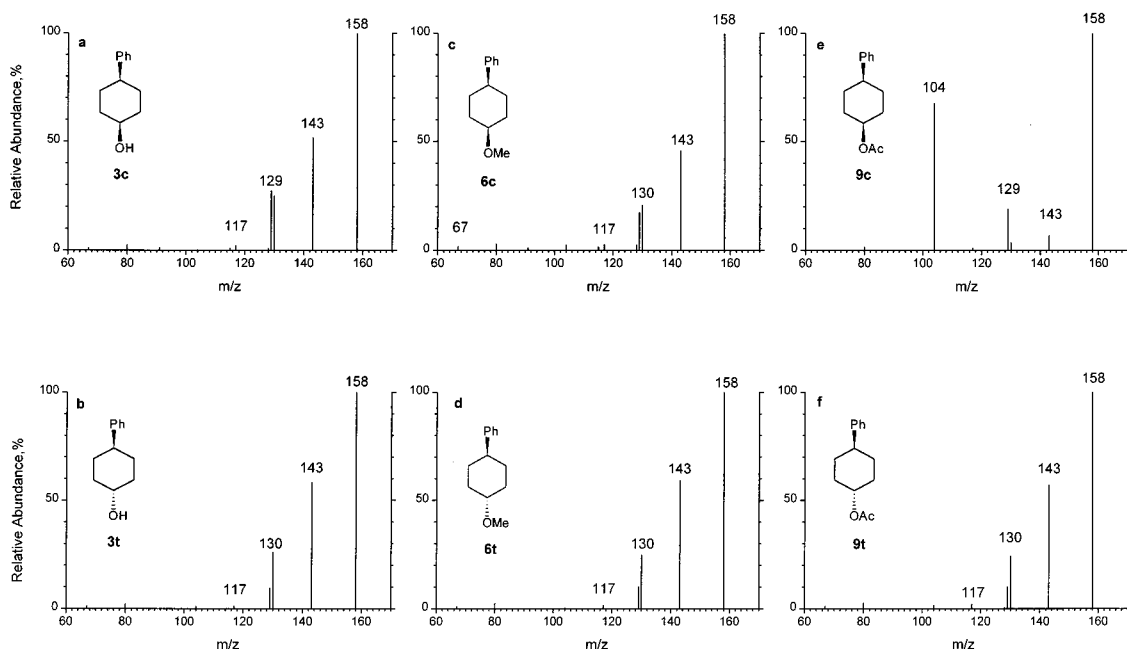
Figure 3. CID spectra (30 eV collision energy, relative ion abundances (%) normalized to the most abundant ion) of the m/z 158 [M - ROH]^+ ions, obtained upon EI from stereoisomeric 4-phenylcyclohexanols and their methyl ethers and acetates: (a) 3c ; (b) 3t ; (c) 6c ; (d) 6t ; (e) 9c ; (f) 9t .
