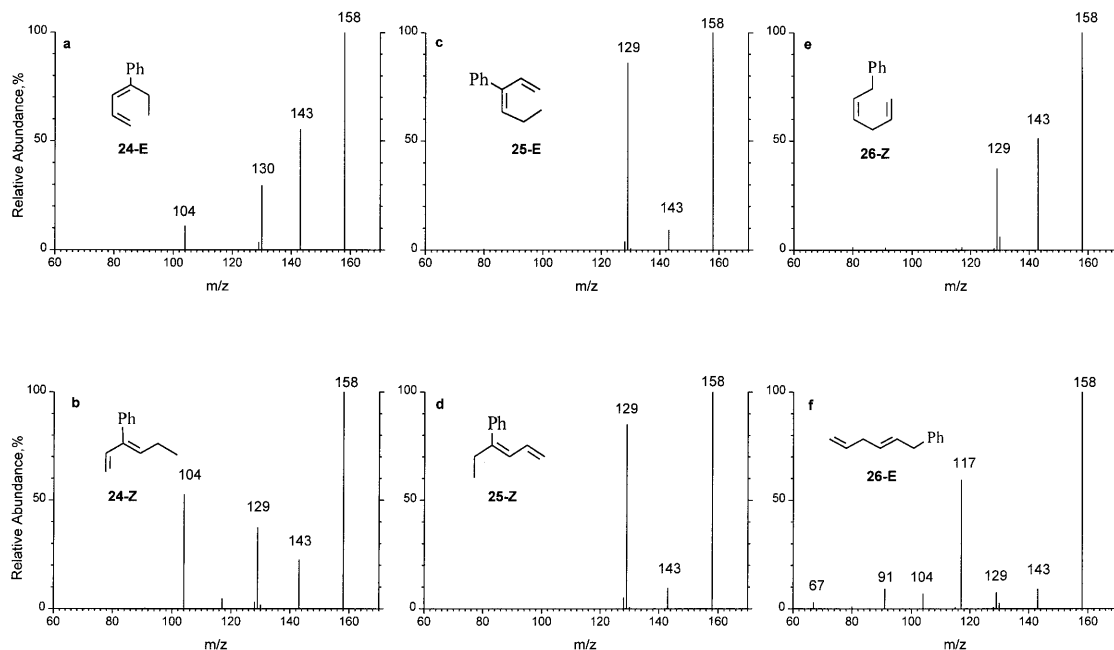
Figure 8. CID spectra (30 eV collision energy, relative ion abundances (%) normalized to the most abundant ion) of the m/z 158 M^{++} ions, obtained upon EI from isomeric phenylhexadienes: (a) 24-E ; (b) 24-Z ; (c) 25-E ; (d) 25-Z ; (e) 26-Z ; (f) 26-E .
