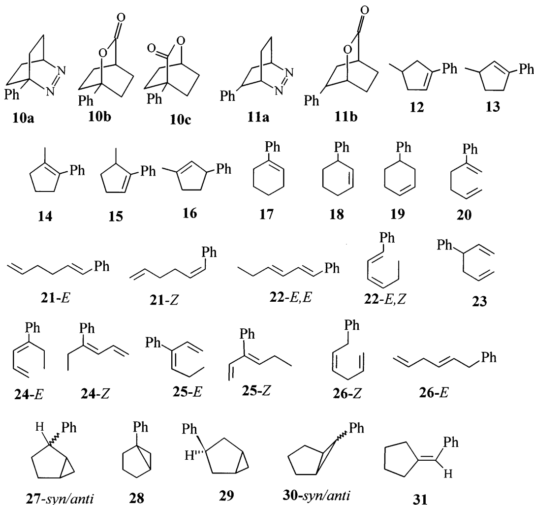
Scheme 3.
