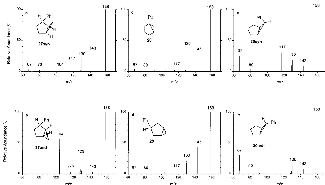
Figure 9. CID spectra (30 eV collision energy, relative ion abundances (%) normalized to the most abundant ion) of the m/z 158 M^{++} ions, obtained upon EI from isomeric phenylbicyclo[3.1.0]hexanes: (a) 27-syn ; (b) 27-anti ; (c) 28 ; (d) 29 ; (e) 30-syn ; (f) 30-anti .
