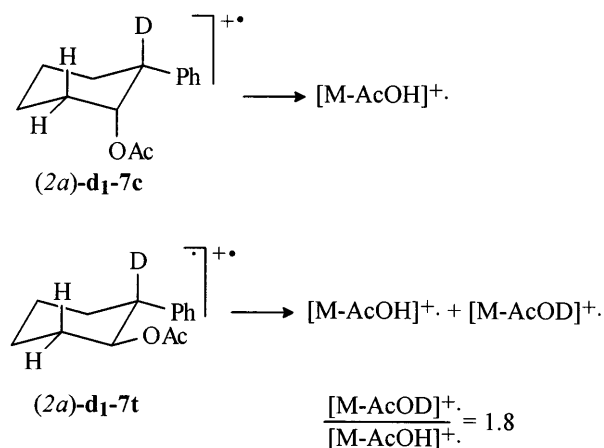
Scheme 15.
