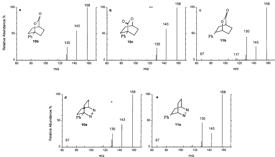
Figure 4. CID spectra (30 eV collision energy, relative ion abundances (%) normalized to the most abundant ion) of the m/z 158 [M - CO_2]^+ and [M - N_2]^+ ions, obtained upon EI from bicyclic lactones and azines: (a) 10b ; (b) 10c ; (c) 11b ; (d) 10a ; (e) 11a .
